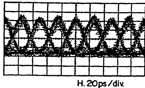
③ 40 Gb/s OPTICAL MUX WAVEFORM
